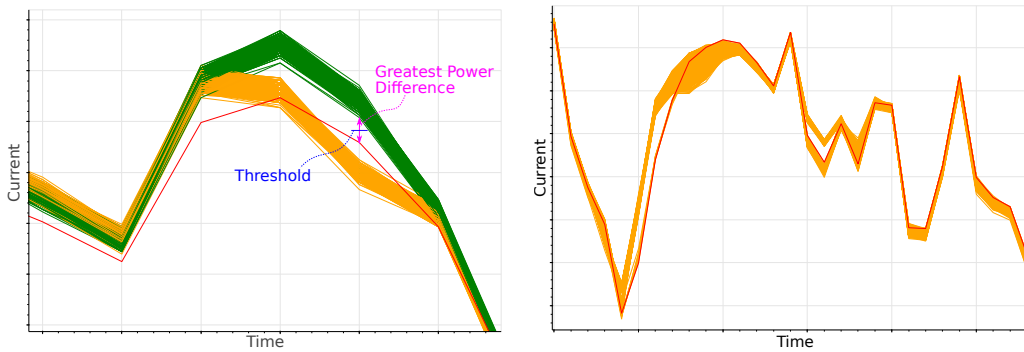
(a) Incorrect recovered bit from POI (in red) for the traditional version. The first 3 iterations have been omitted for clarity. (b) Missed ROI (in red) compared to the other ROI for the 50-sample pattern and the windowed version.
