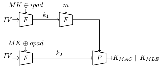
Figure 2: Key generation using HMAC.
